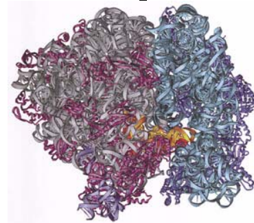
Ribozyme
