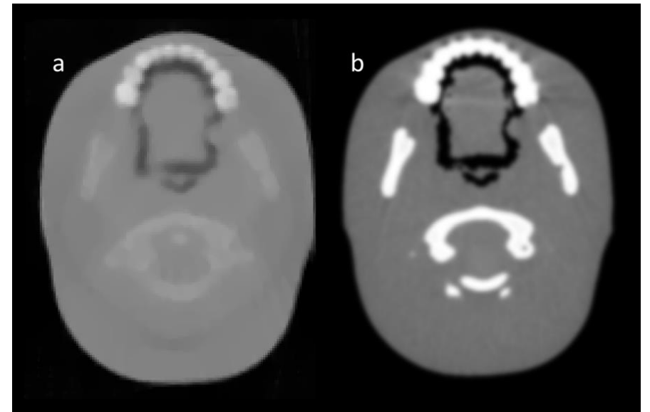
proton CT
