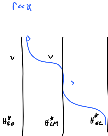
FIG. 5. Low-lying energy levels of H_N as a function of odd N for U/D = 10^{-3} , U/\pi\Gamma = 12.66 , and \Lambda = 2.5 . On the left-hand vertical scale are the lowest-lying free-orbital fixed-point levels for N odd, while on the right-hand side are the equivalent levels for N even. The following fixed-point regimes obtain: free orbital 5 < N < 15 , local moment 23 < N < 51 , strong coupling 61 < N .
