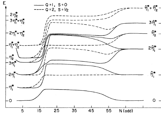
FIG. 5. Low-lying energy levels of H_N as a function of odd N for U/D = 10^{-3} , U/\pi\Gamma = 12.66 , and \Lambda = 2.5 . On the left-hand vertical scale are the lowest-lying free-orbital fixed-point levels for N odd, while on the right-hand side are the equivalent levels for N even. The following fixed-point regimes obtain: free orbital 5 < N < 15 , local moment 23 < N < 51 , strong coupling 61 < N .
